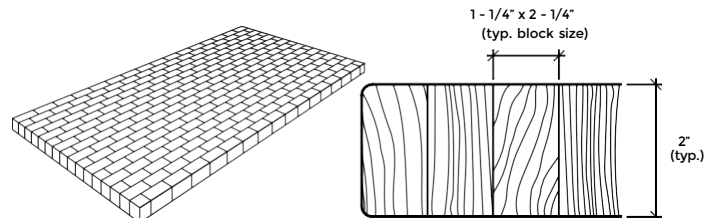
END GRAIN
