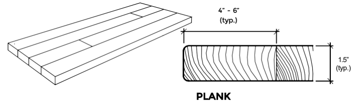
PLANK
