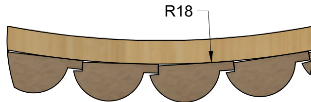
DETAIL B SCALE 6" = 1'-0"
