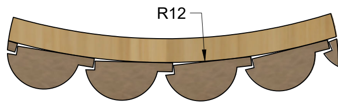
DETAIL A SCALE 6" = 1'-0"
