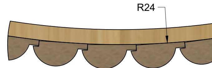
DETAIL C SCALE 6" = 1'-0"
